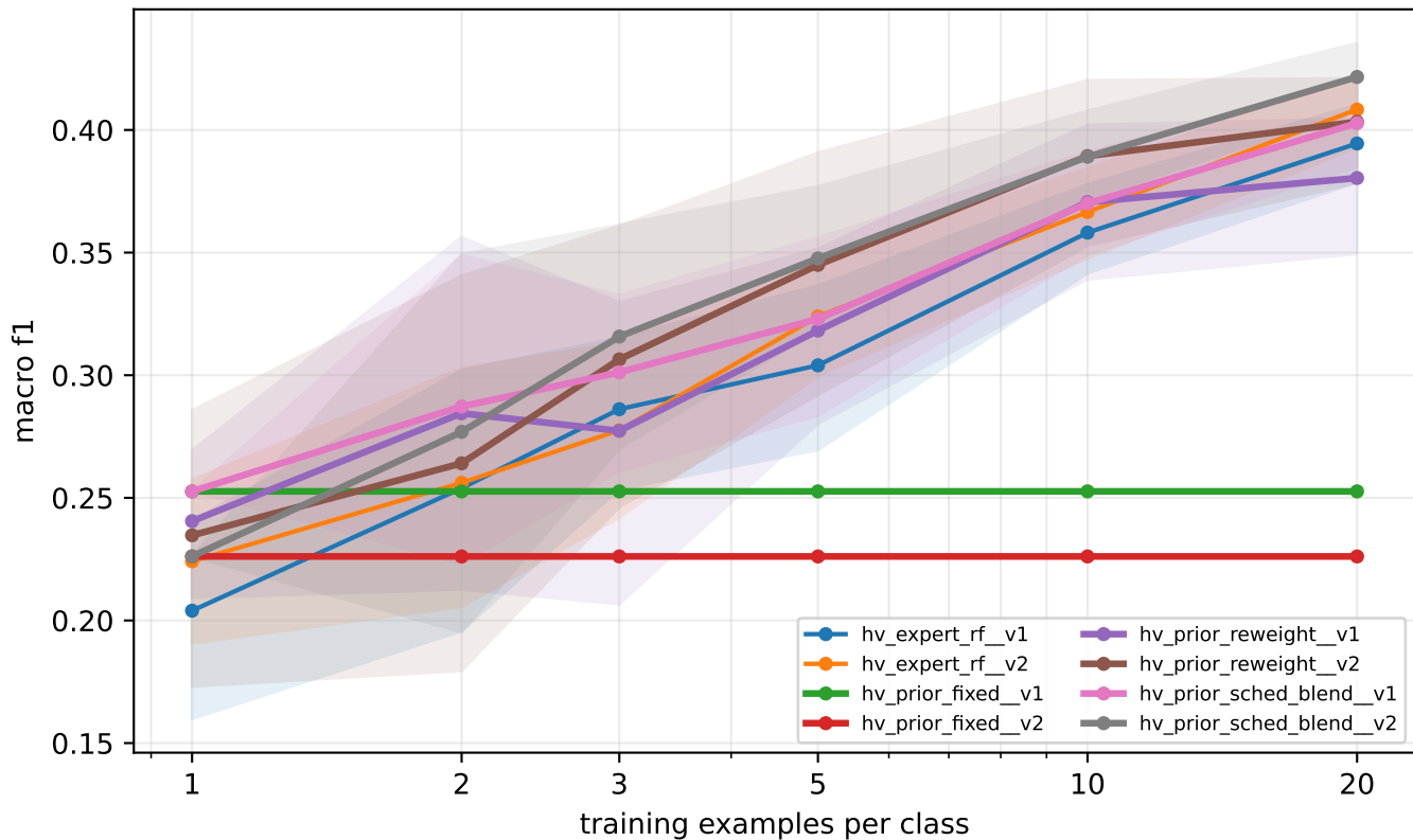
GoEmotions: prior wording v1 vs v2 (identical tau=4)
