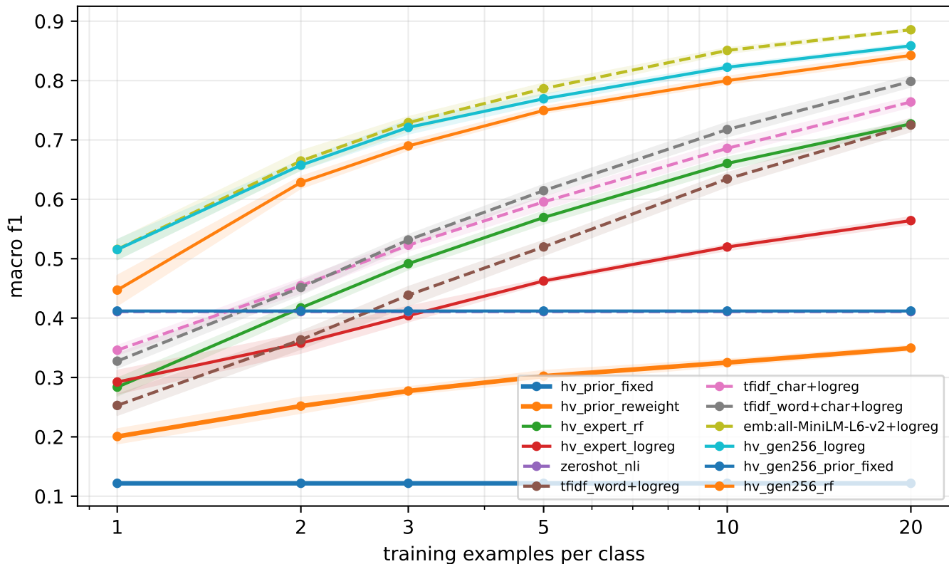
Banking77: 24 expert vs 256 generated hypotheses
