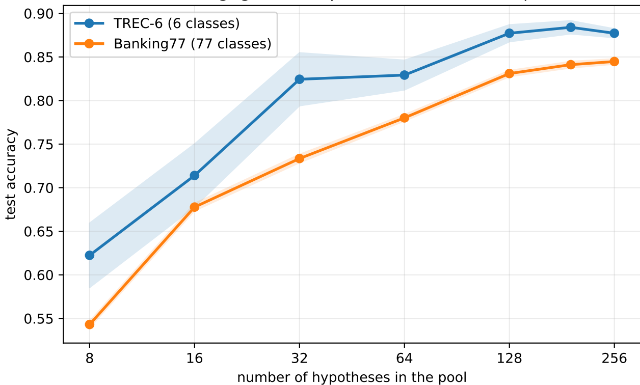
Pool-size scaling (generated pool, RF head, 20 examples/class)
