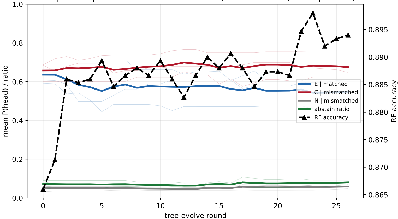
trec: per-head profile across tree-evolve rounds (mean of 3 seeds; thin = per seed)
