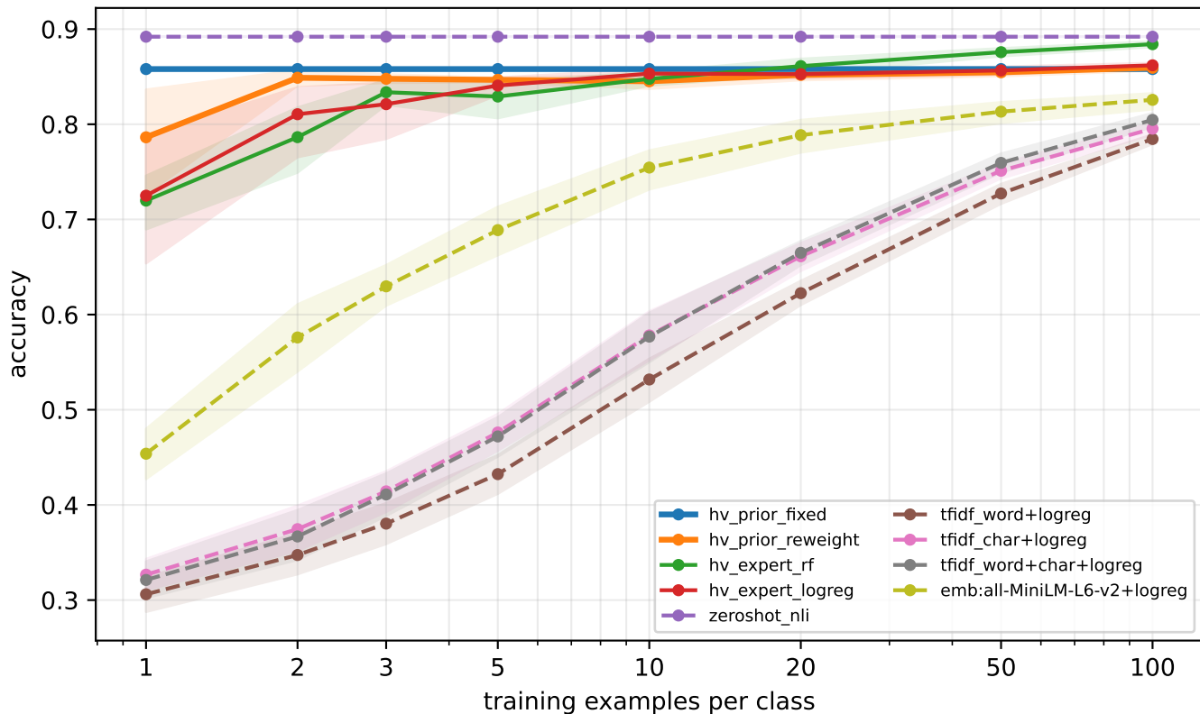
AG News low-label learning curve (finecat-nli-l)
