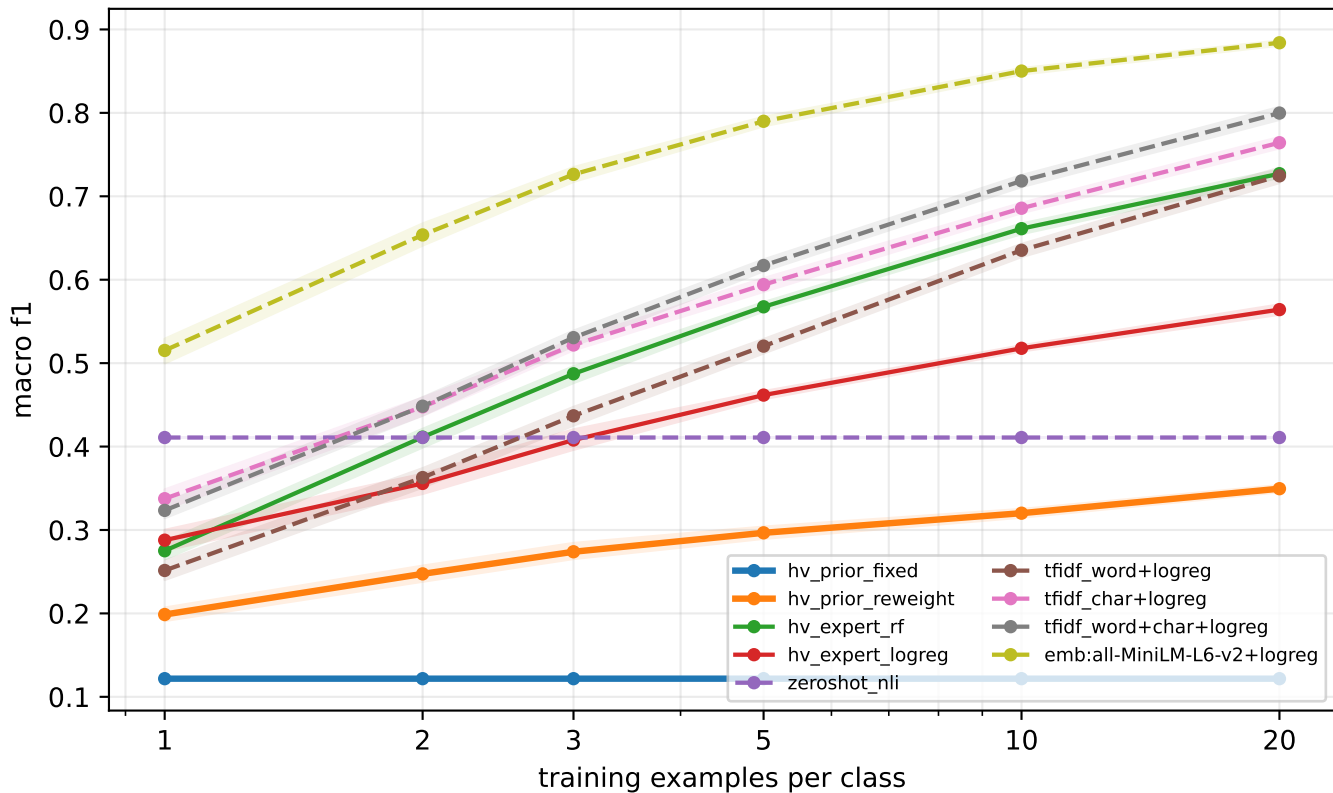
Banking77 low-label learning curve (finecat-nli-l)
