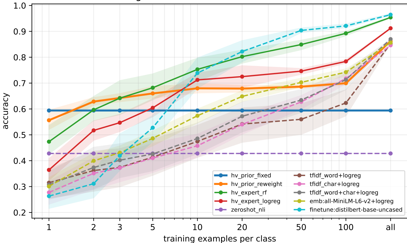
TREC-6 learning curve: HV vs baselines vs fine-tuned DistilBERT
