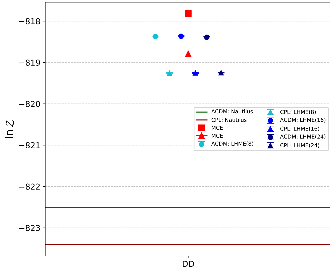
Individual evidences (DD)
