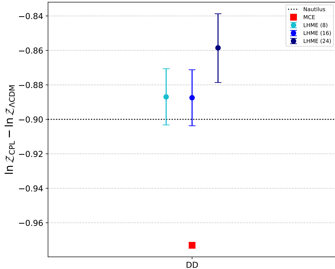
Bayes factor (DD)
