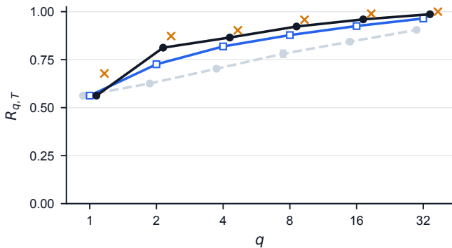
(c) Cycle-basis 2-cells
