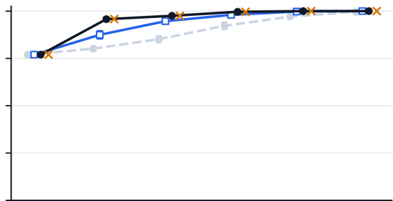
(b) 2-simplices
