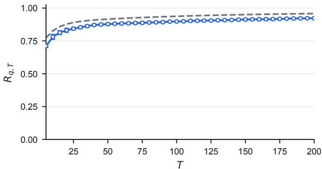
(c) Cycle-basis 2-cells
