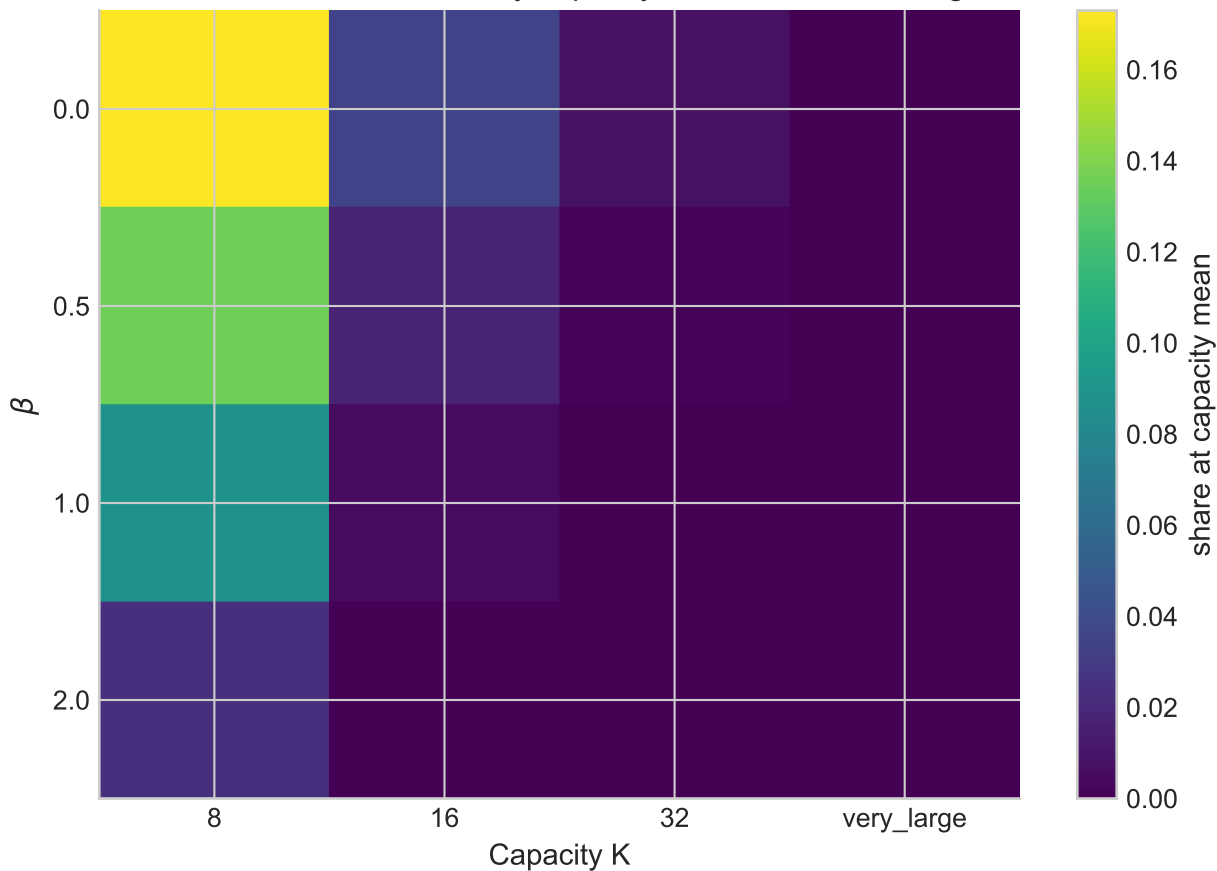
Share of saturated nodes by capacity and saturation strength
