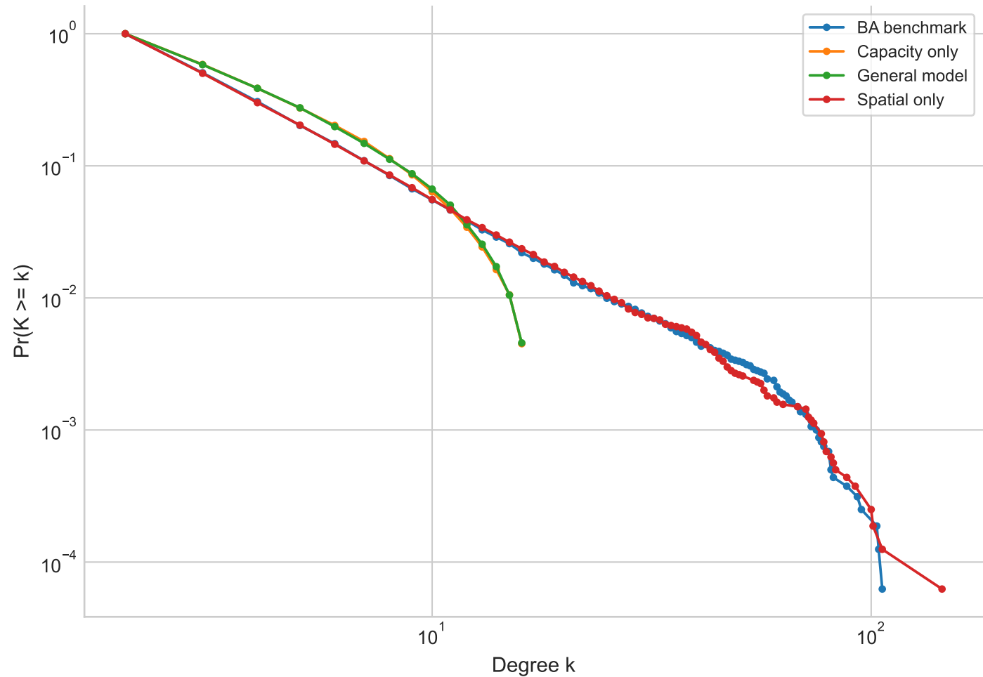
Degree CCDF by headline scenario
