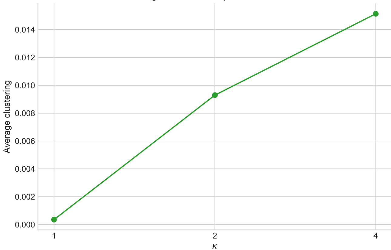
Clustering rises with multiple initial attachments
