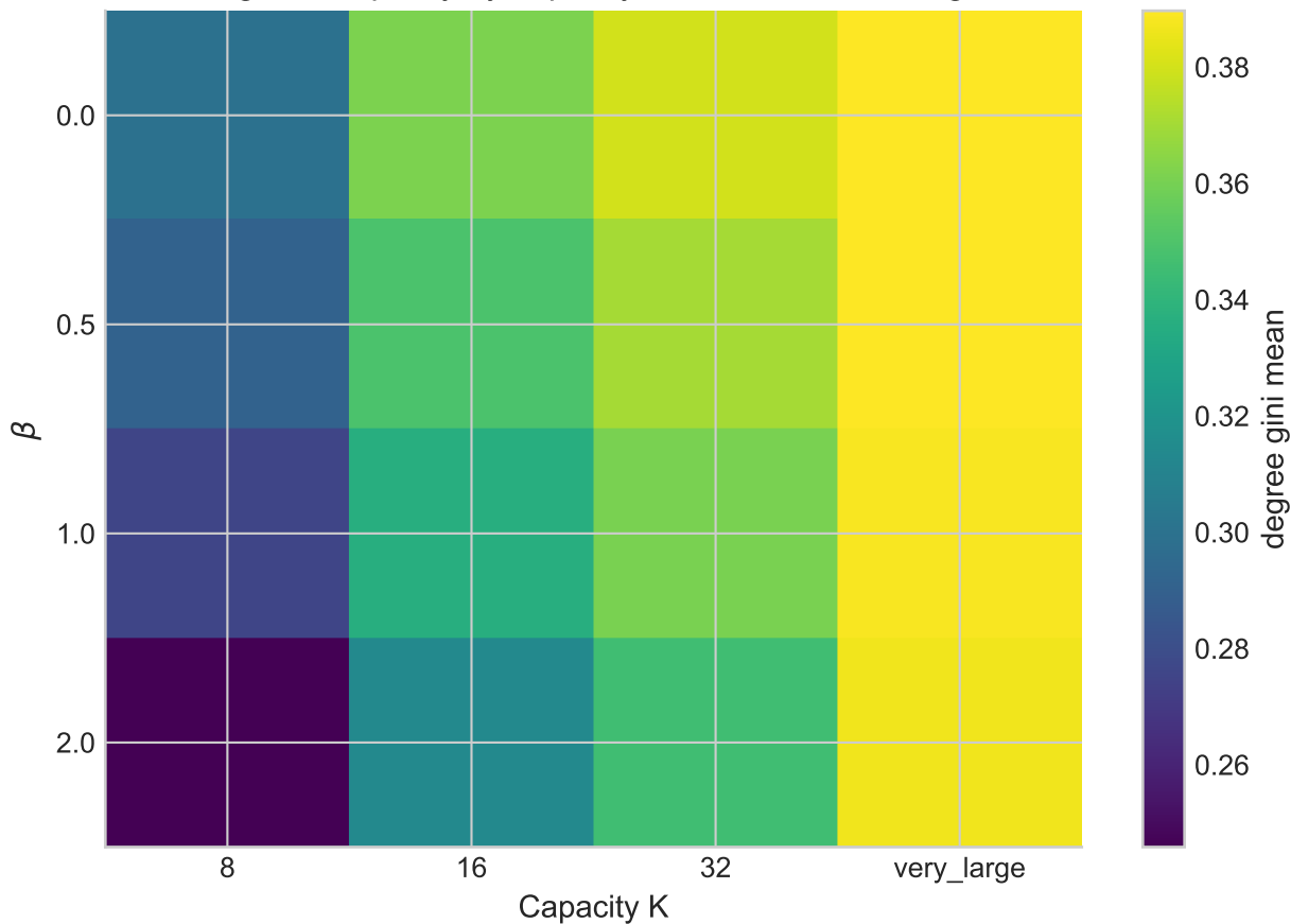
Degree inequality by capacity and saturation strength
