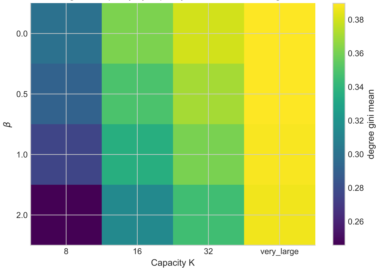
Degree inequality by capacity and saturation strength
