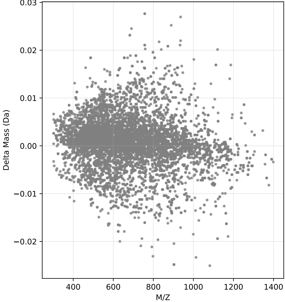
M/Z vs Delta Mass
