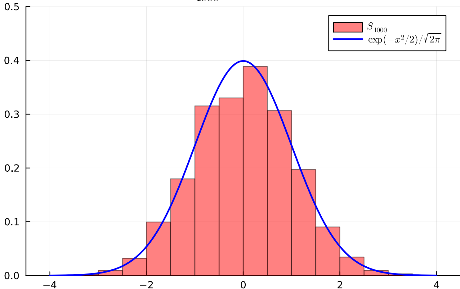
Histogram of S_{1000} , sampled 10000 times
