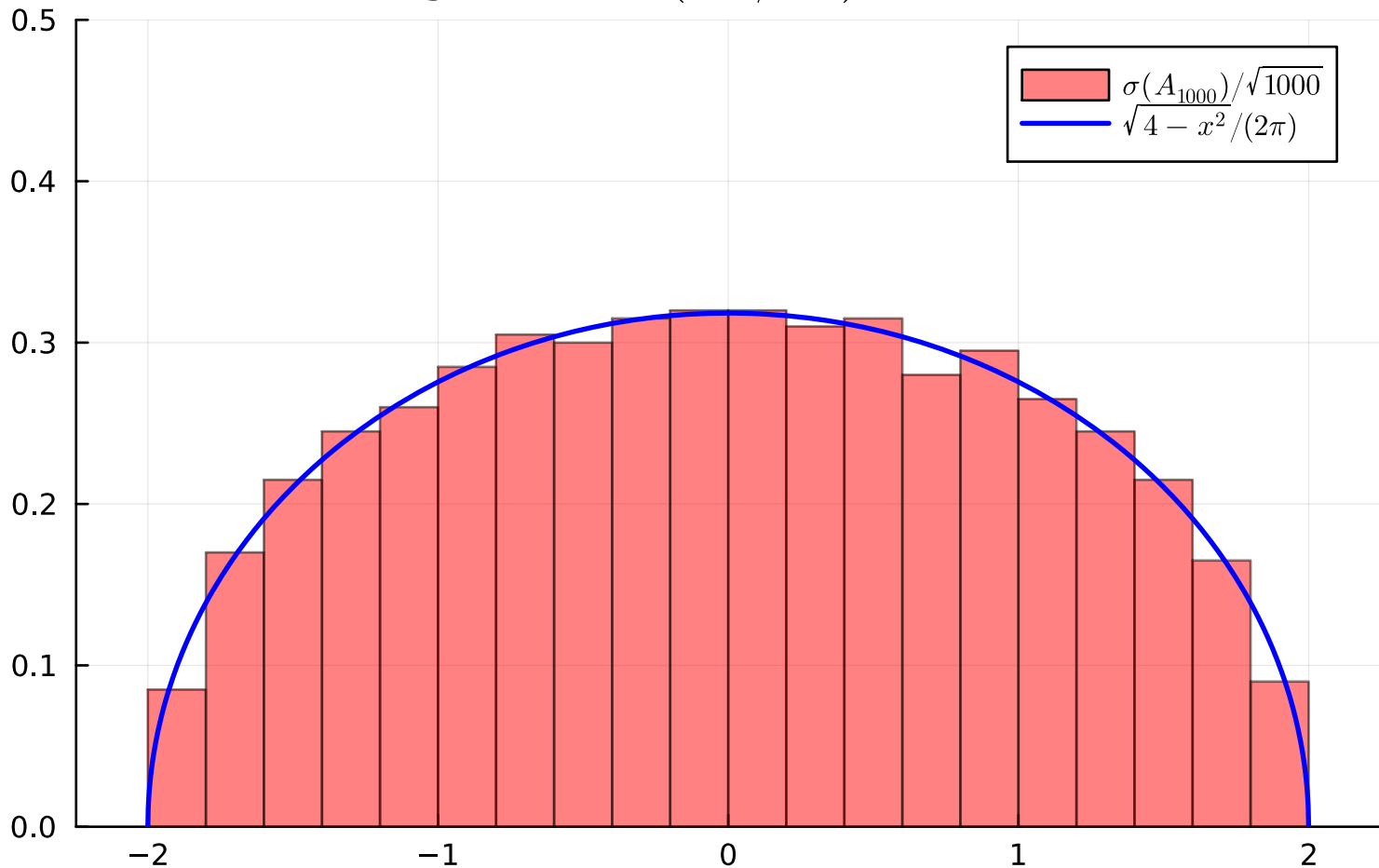
Histogram of \sigma(A_n/\sqrt{n}) for n = 1000
