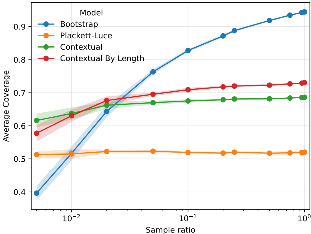
Coverage vs. Sample Ratio by Model
