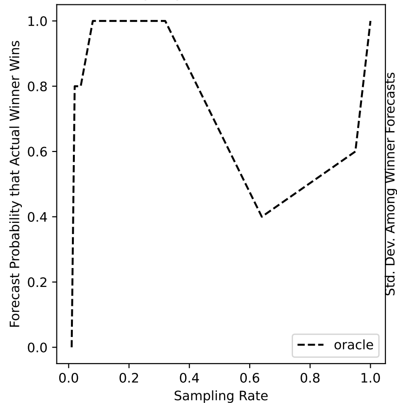
glasgow-01 Forecast
