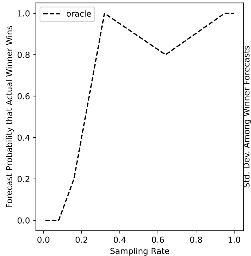
glasgow-05 Forecast
