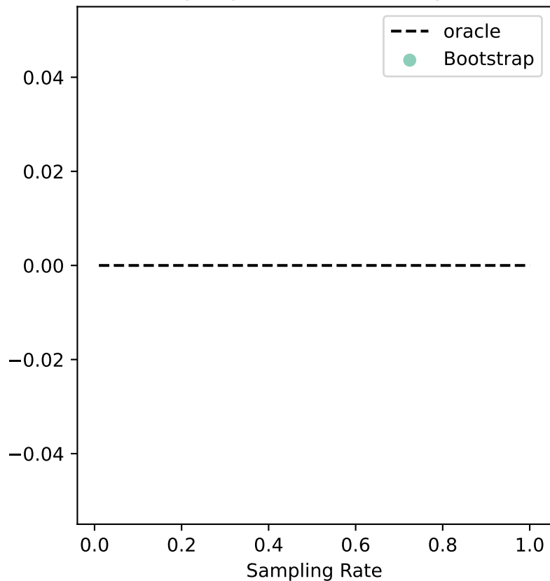
glasgow-12 Uncertainty
