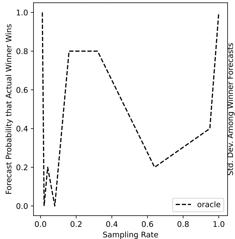
glasgow-12 Forecast
