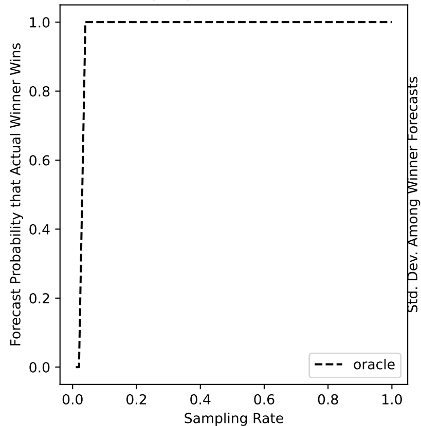
glasgow-13 Forecast
