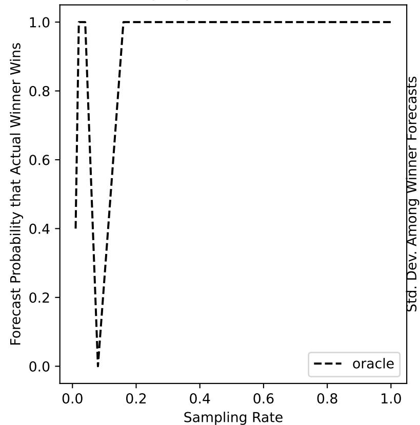
glasgow-15 Forecast
