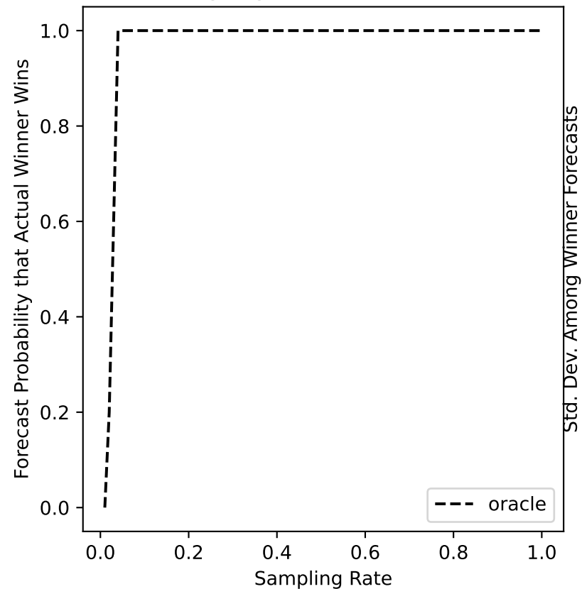
glasgow-19 Forecast
