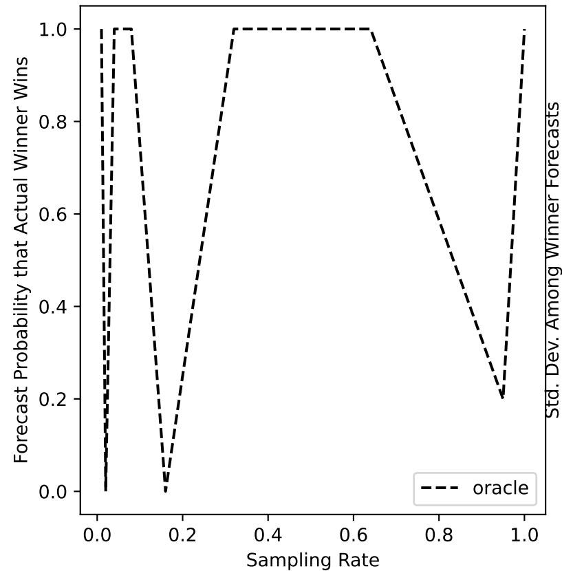
glasgow-20 Forecast
