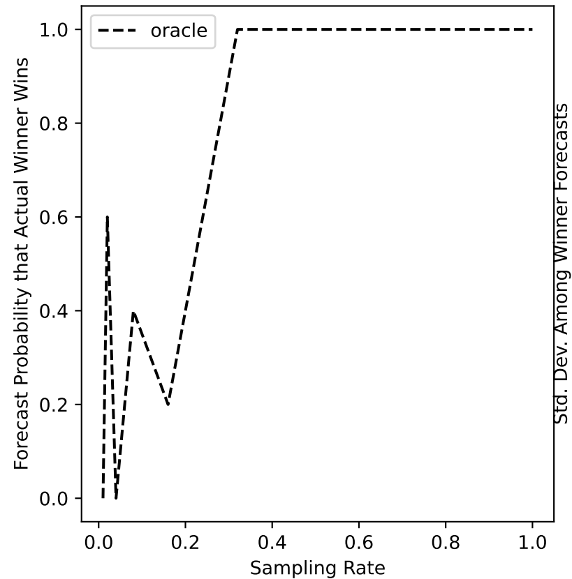
uklabor-01 Forecast
