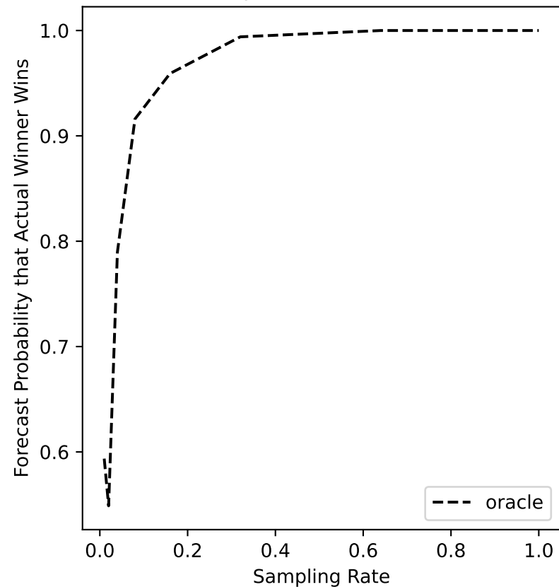
aspen-02 Forecast
