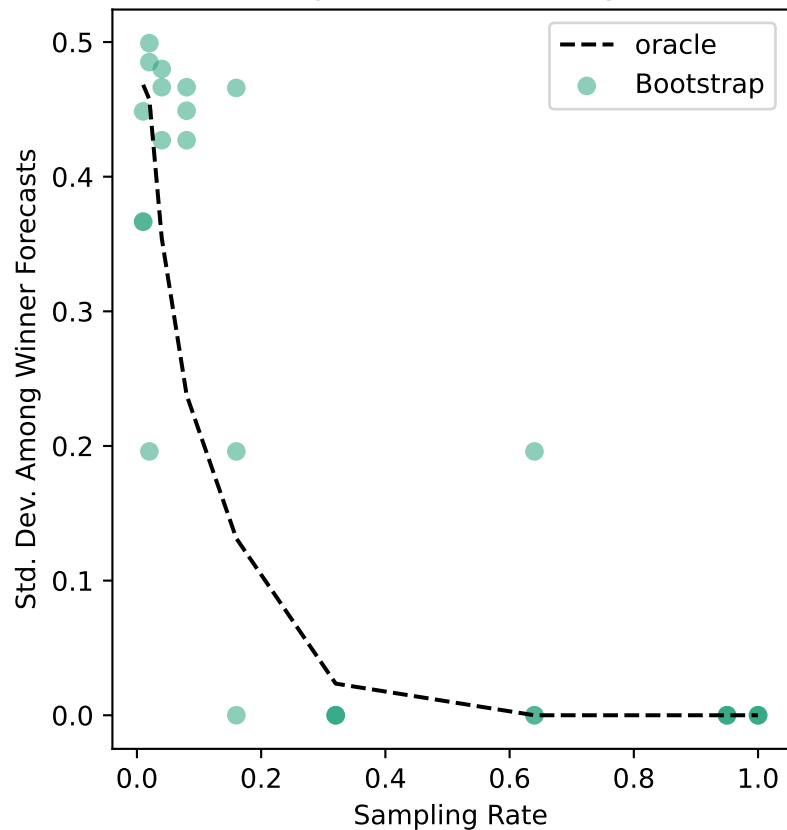
aspen-02 Uncertainty
