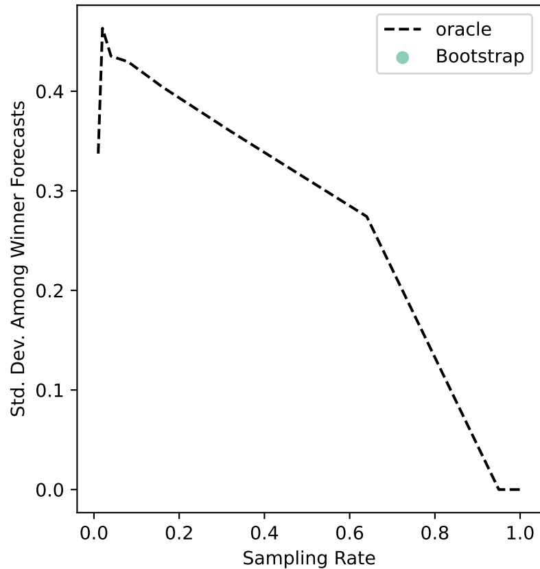
debian-04 Uncertainty
