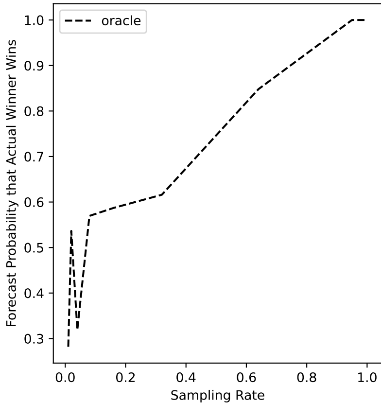
debian-04 Forecast
