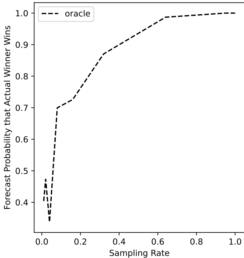
debian-05 Forecast
