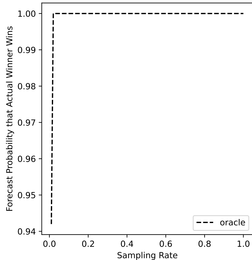
debian-07 Forecast
