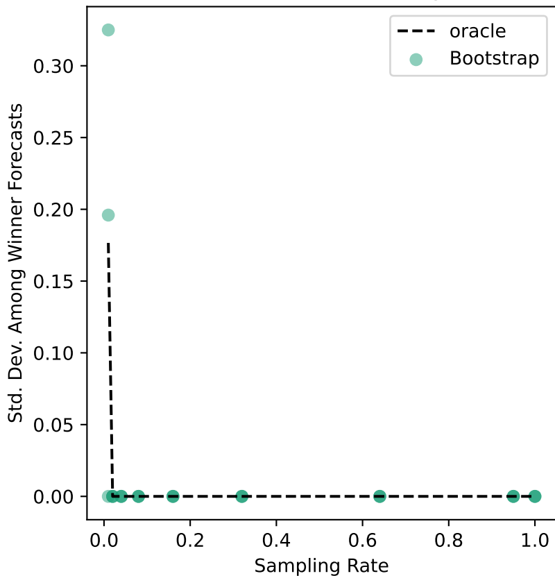
debian-07 Uncertainty
