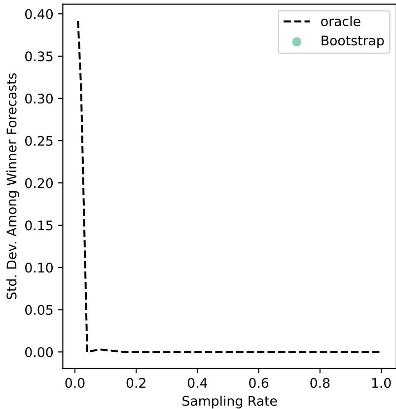
ers-03 Uncertainty
