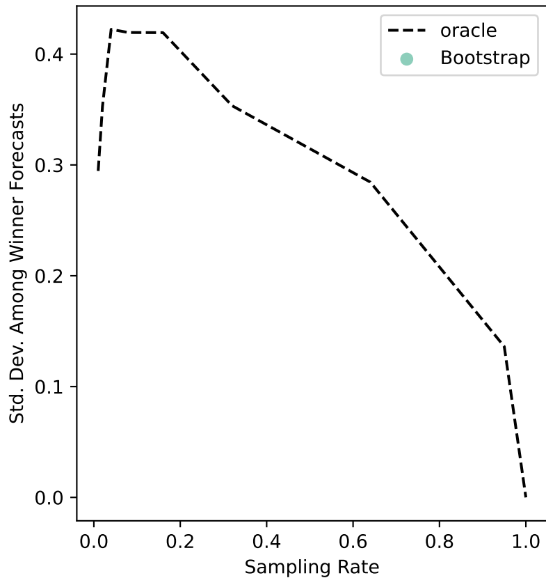
ers-14 Uncertainty
