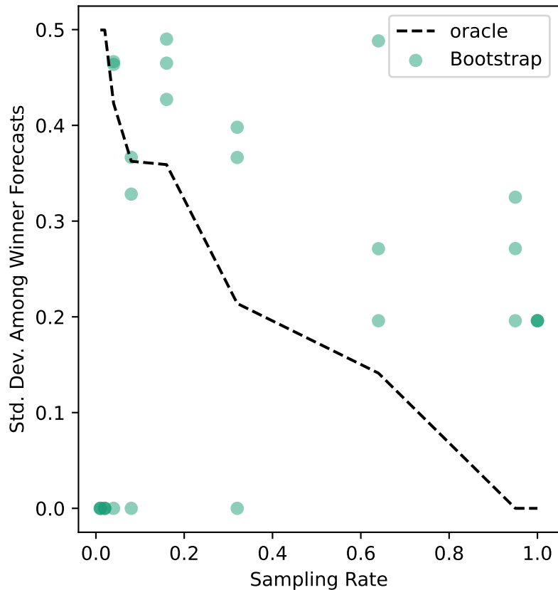
ers-17 Uncertainty
