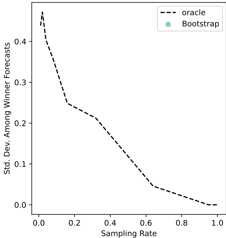
ers-43 Uncertainty
