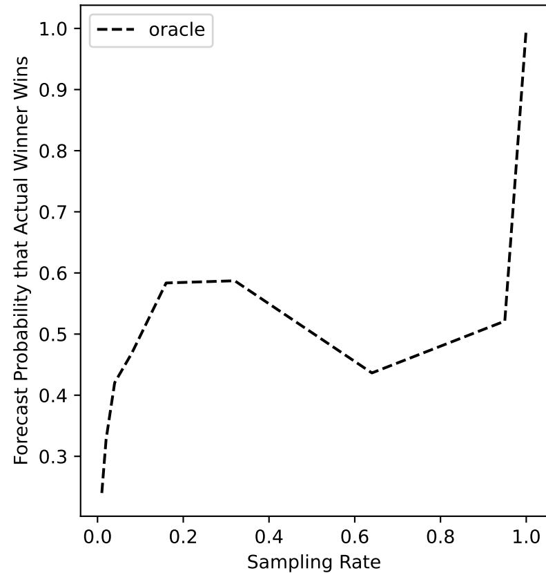
ers-52 Forecast
