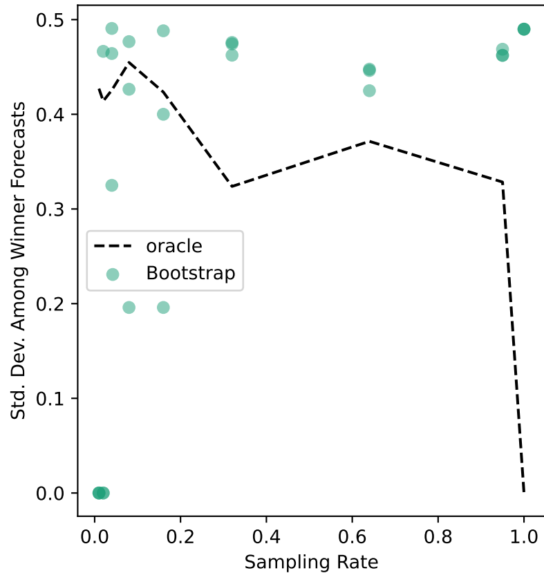
ers-52 Uncertainty
