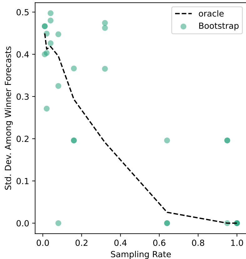
ers-61 Uncertainty
