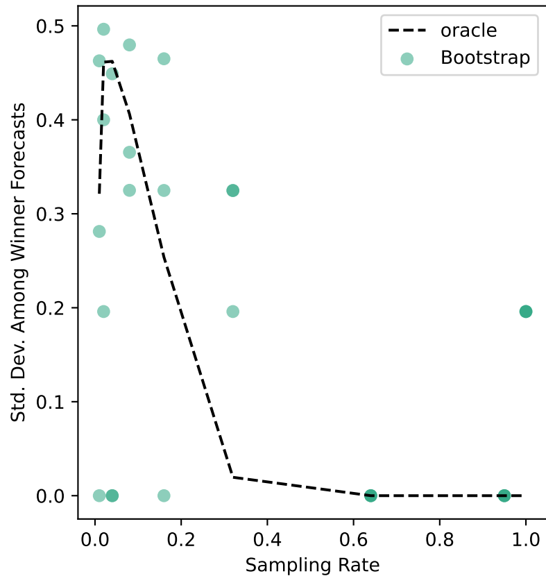
ers-71 Uncertainty
