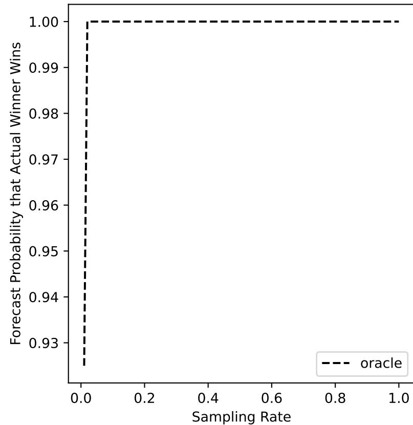
glasgow-03 Forecast
