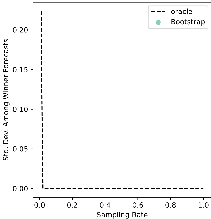
glasgow-03 Uncertainty
