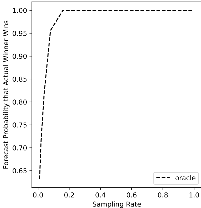
glasgow-13 Forecast
