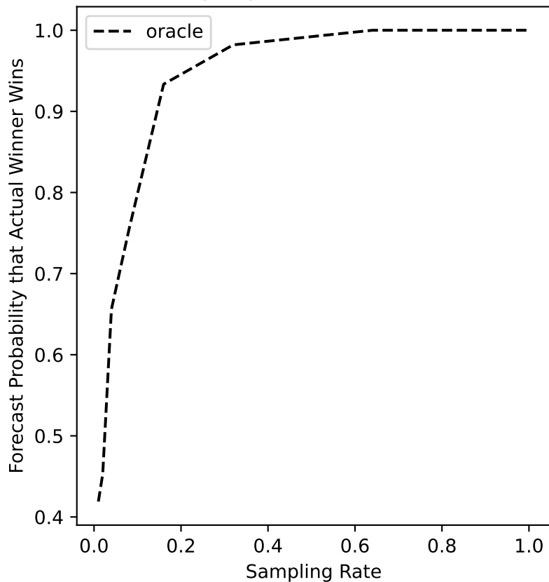
glasgow-15 Forecast
