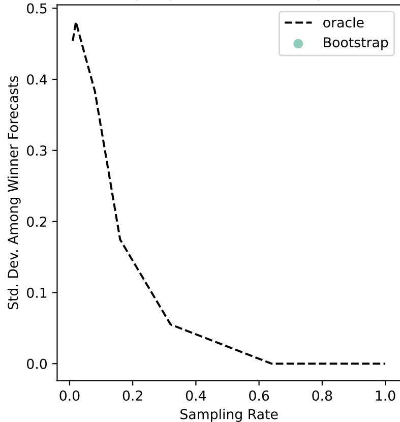
glasgow-15 Uncertainty
