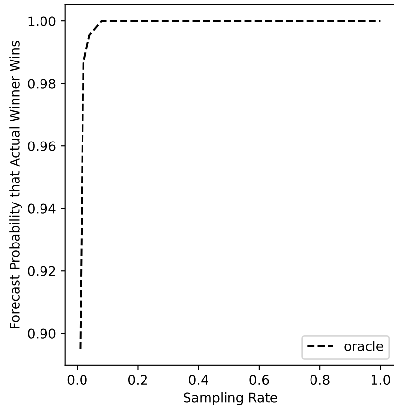
glasgow-16 Forecast
