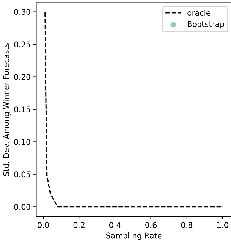
glasgow-16 Uncertainty
