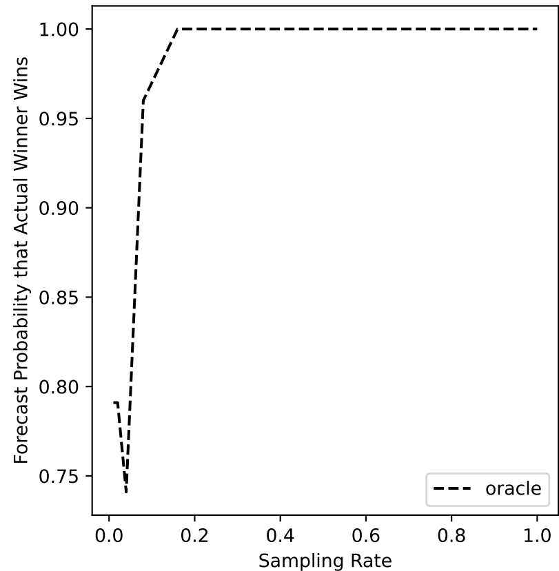
minneapolis-02 Forecast
