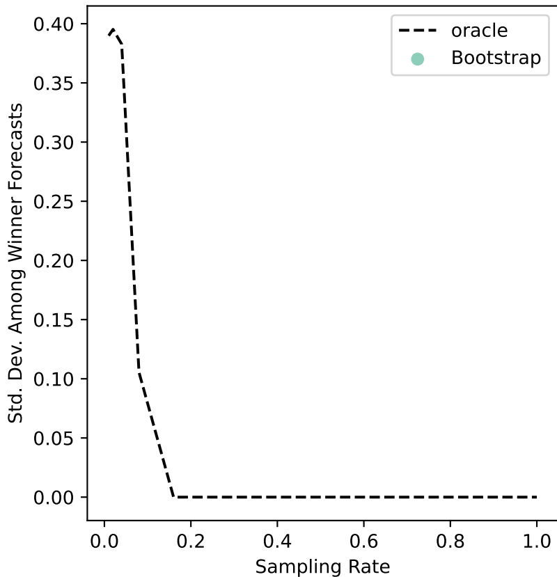
minneapolis-02 Uncertainty
