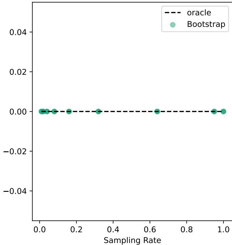
oakland-01 Uncertainty
