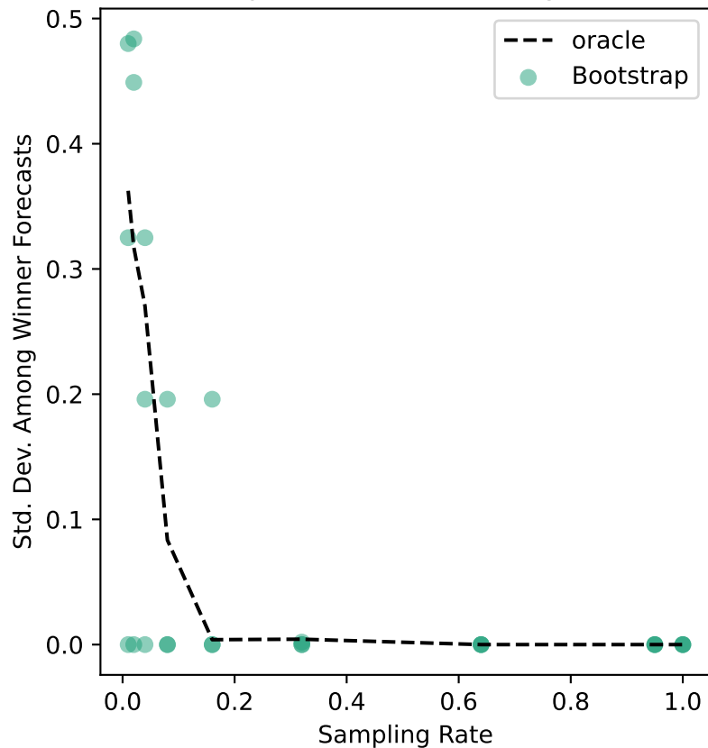
pierce-04 Uncertainty
