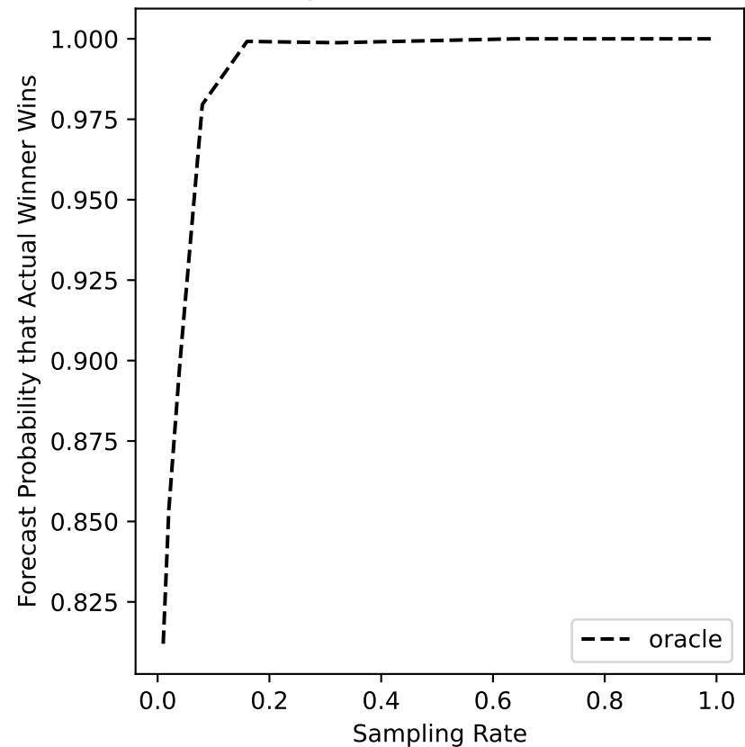
pierce-04 Forecast
