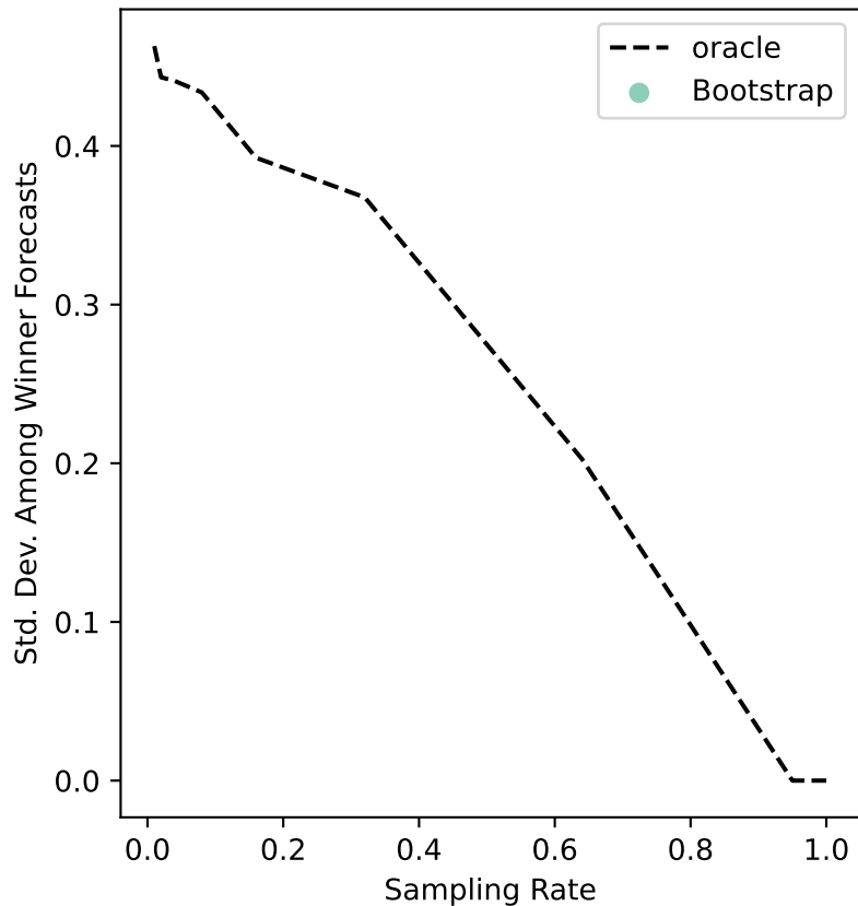
sf-14 Uncertainty
