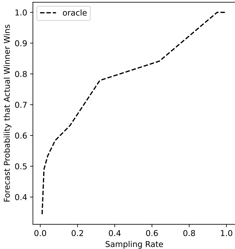
uklabor-01 Forecast
