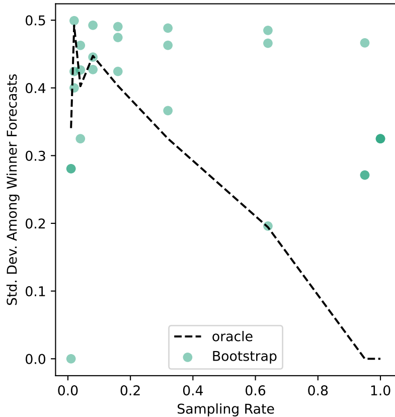
uklabor-01 Uncertainty
