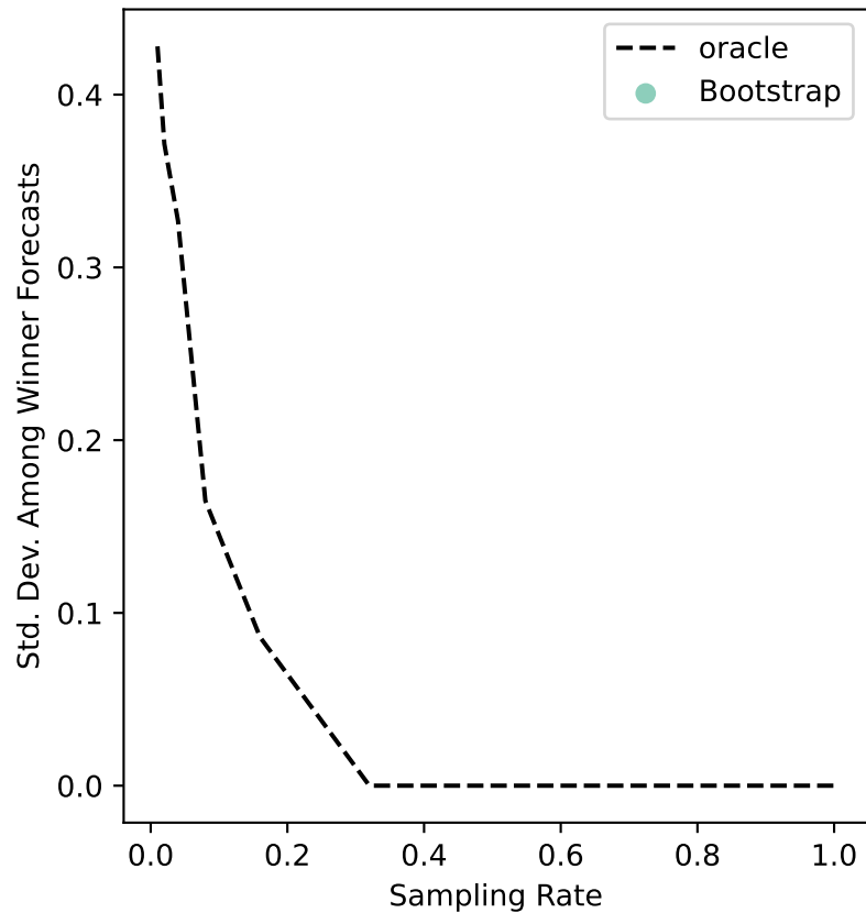
apa-05 Uncertainty
