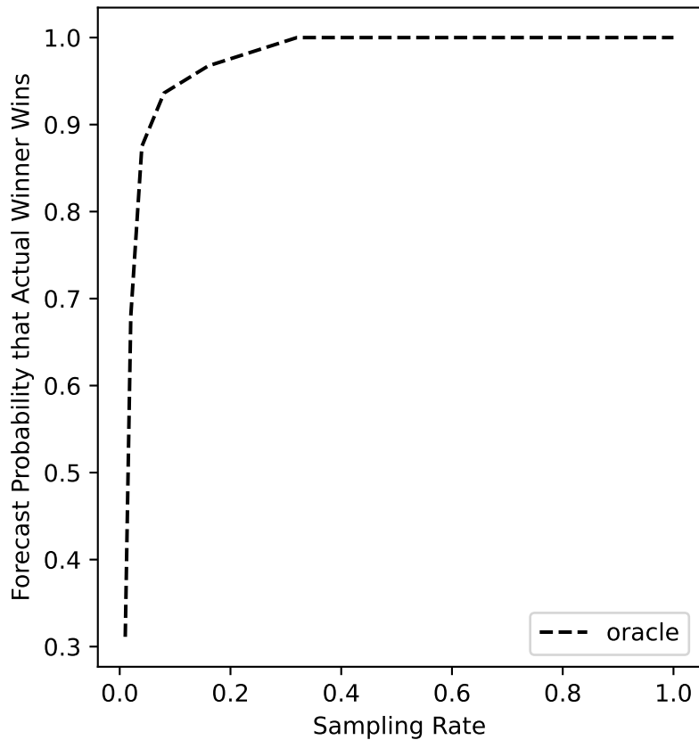
apa-05 Forecast
