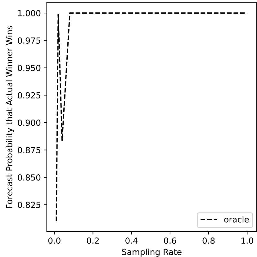
debian-06 Forecast
