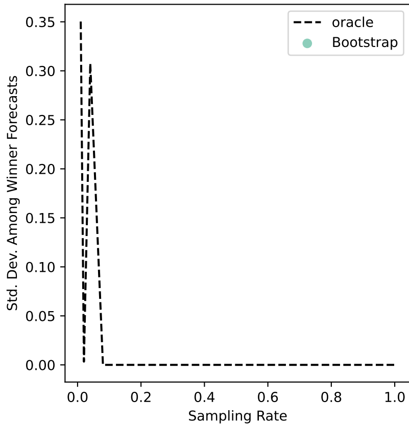
debian-06 Uncertainty
