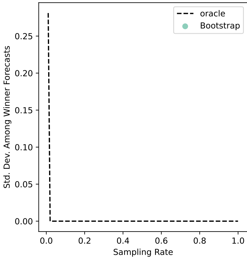
ers-03 Uncertainty
